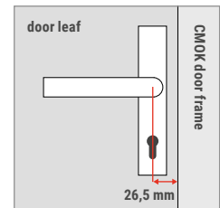
3. Handle and rosette dimensions. Door handle cannot extend beyond the spindle.
