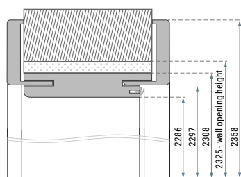
Dimensions of door frame for PN23 door.
