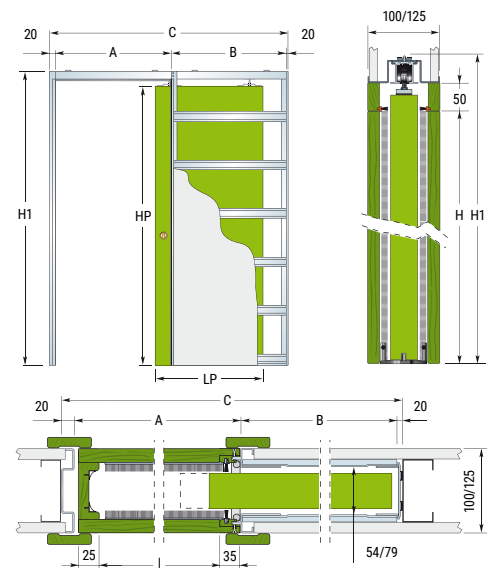
SINGLE POCKET DIMENSION TABLE
