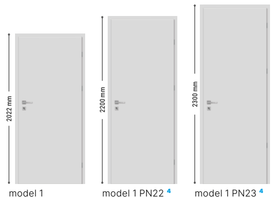
Dimensions of door frame for PN23 door.
