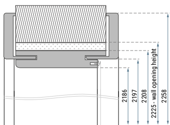
Dimensions of door frame for PN22 door.
