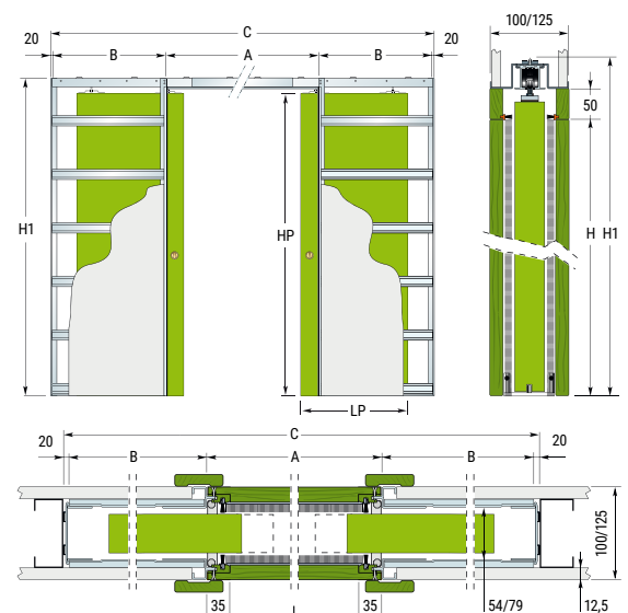
DOUBLE POCKET DIMENSION TABLE
